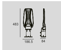
LMR02-100W
