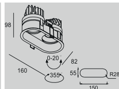
LM102033
