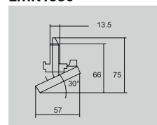
LMK1550
