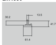
LM1550
